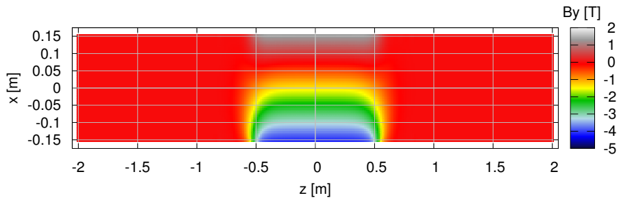
Figure 67. Vertical component of the magnetic field on the median plane of the F magnet obtained with the ROXIE code.
