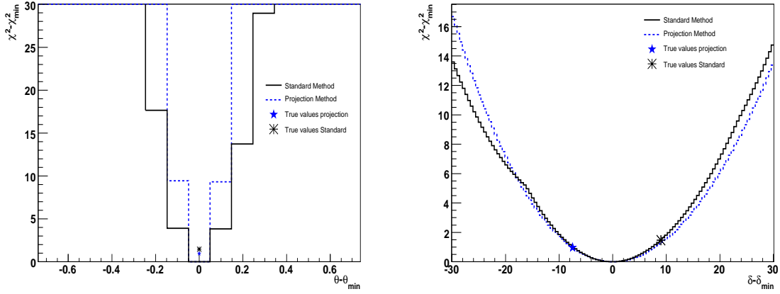
Figure 136. Projection of the minimum \chi^2 onto the \theta_{13} axis (left) and the \delta axis (right) for \theta_{13} = 1^\circ and \delta = 45^\circ .
