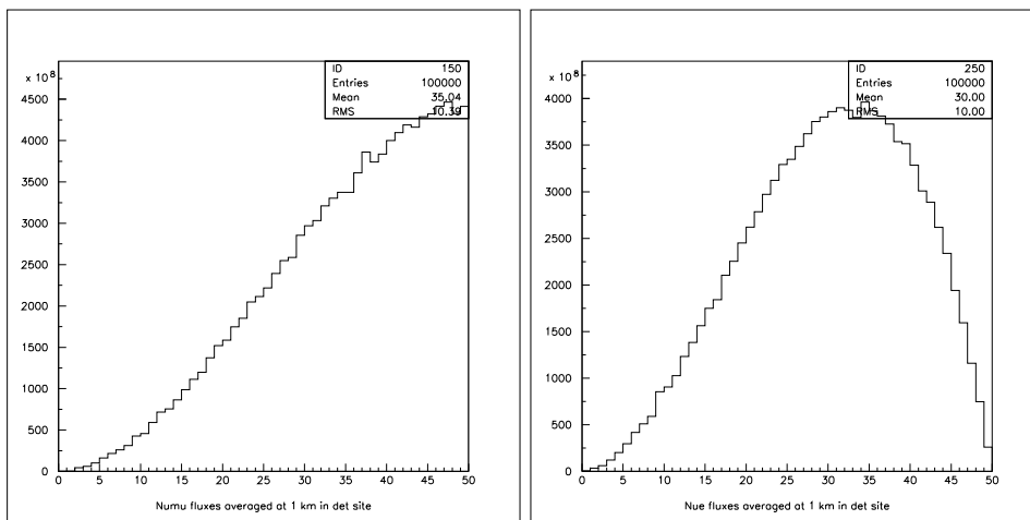
Figure 9: Flux of \bar{\nu}_\mu (left panel) and \nu_e (right panel) at a detector 2500 km from a neutrino factory with a 20 m radius, subtending an angle of 8 \mu\text{rad} ., from the decay of 50 GeV \mu^+ .
